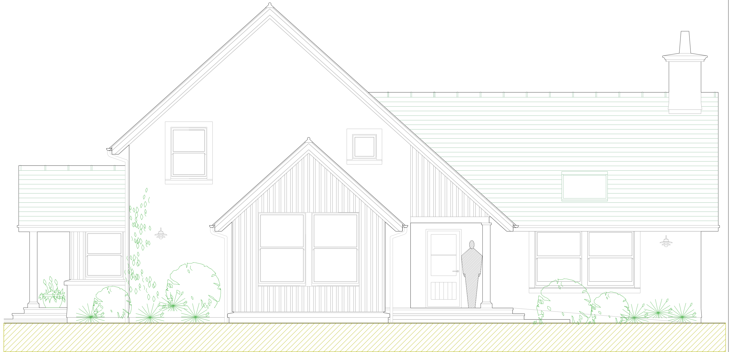
SOUTH WEST ELEVATION
